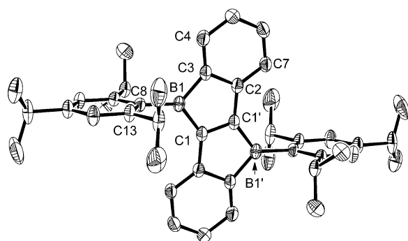
Figure 3. Thermal ellipsoid (50%) diagrams of the molecular structure of 3 . Selected bond lengths [ \text{\AA} ], angles [ ^\circ ], and dihedral angles [ ^\circ ]: \text{C1-B1} 1.571(4), \text{C1-C1'} 1.367(5), \text{C1'-C2} 1.480(4), \text{C2-C3} 1.419(3), \text{C3-B1} 1.588(4), \text{C3-B1-C1} 102.1(2) , \text{C8-B1-C1} 128.6(2) , \text{C8-B1-C3} 129.2(2) , \text{C1-B1-C8-C13} -90.1(4) , \text{C1-C1'-C2-C3} 0.1(4) .
